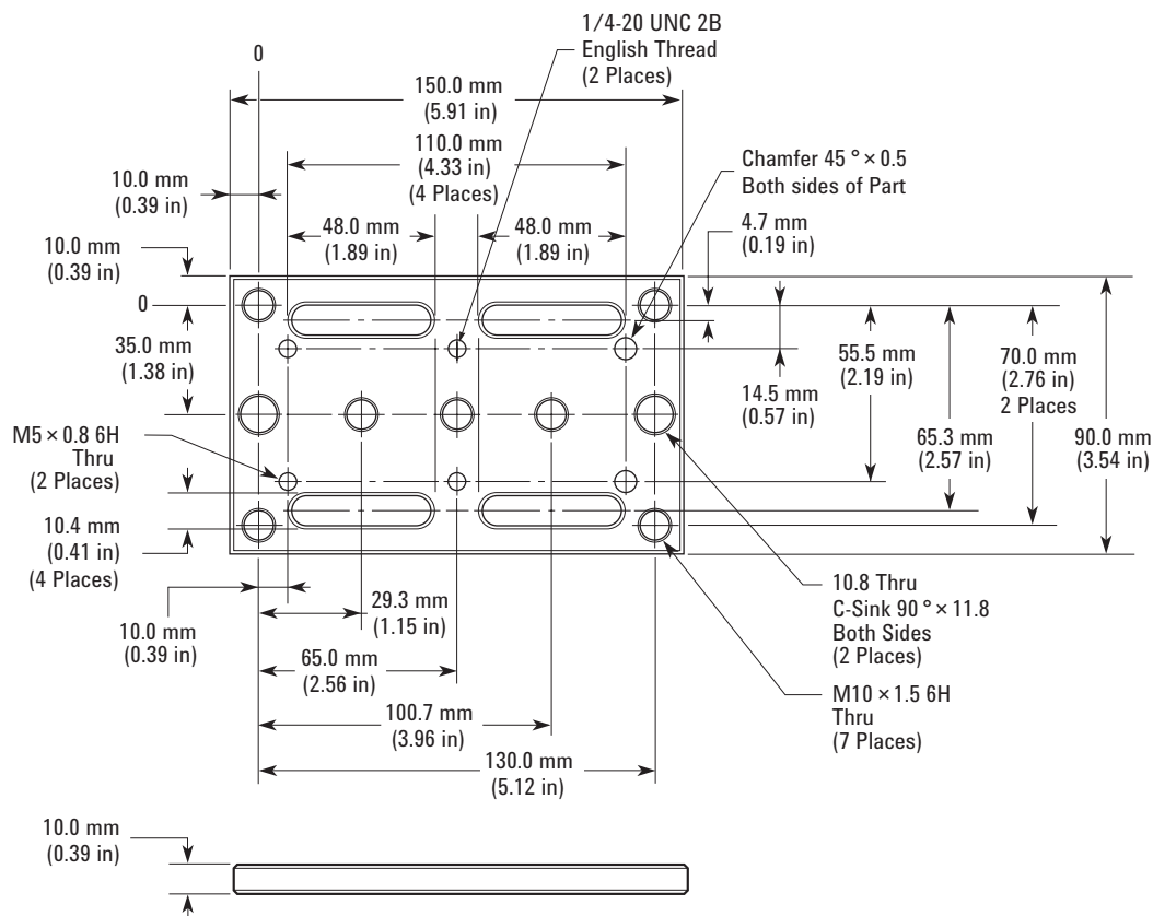
Keysight 10768-20214 Base - Large
