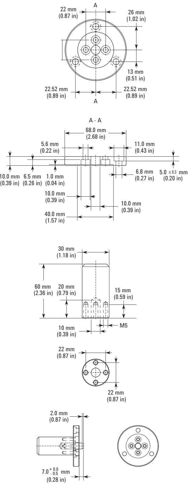
Flanged Shaft
