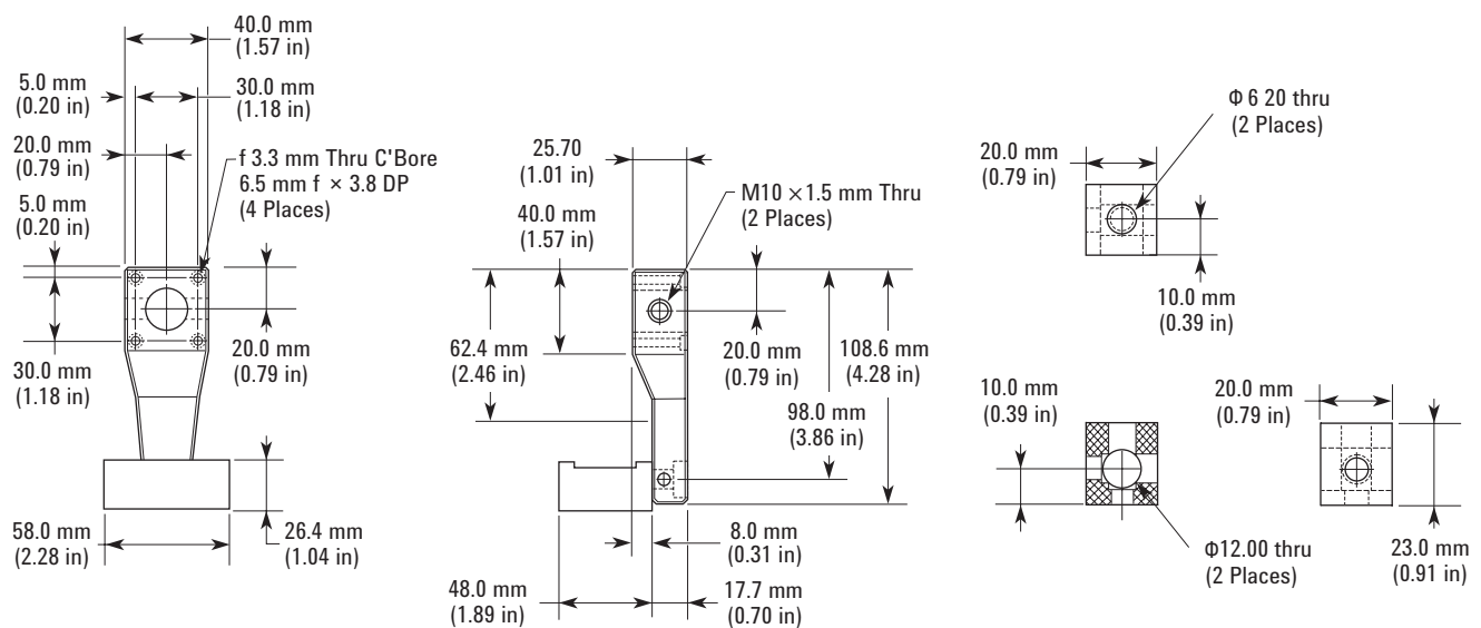
Keysight 10769B Turning Mirror (Base Block Only)
