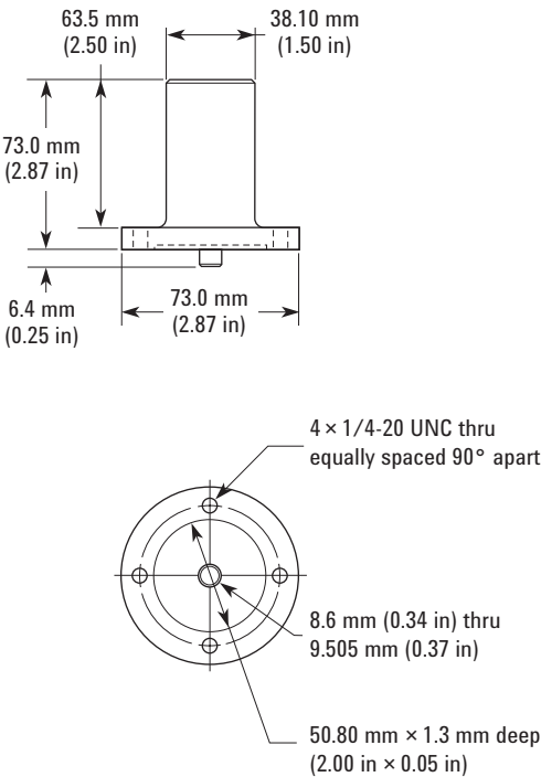
Flanged Shaft
