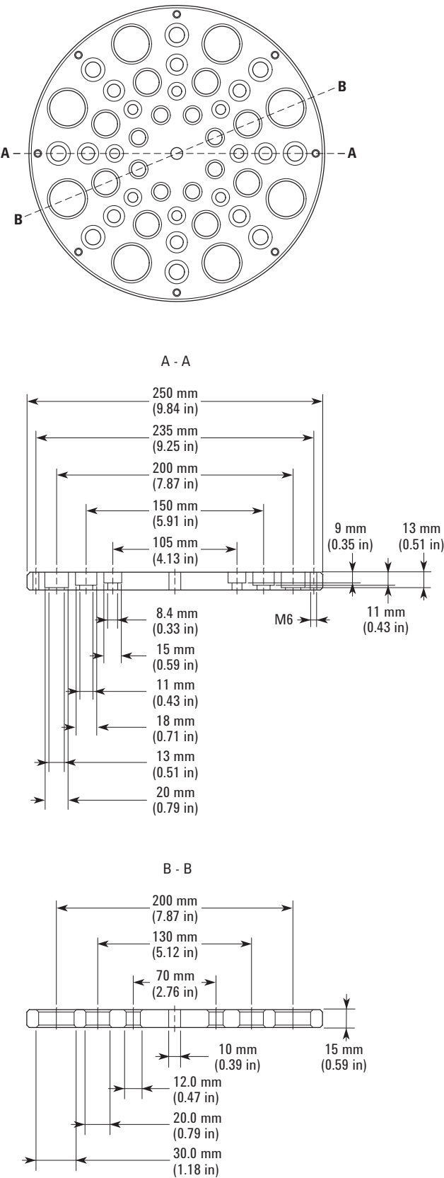
Adapter Plate
